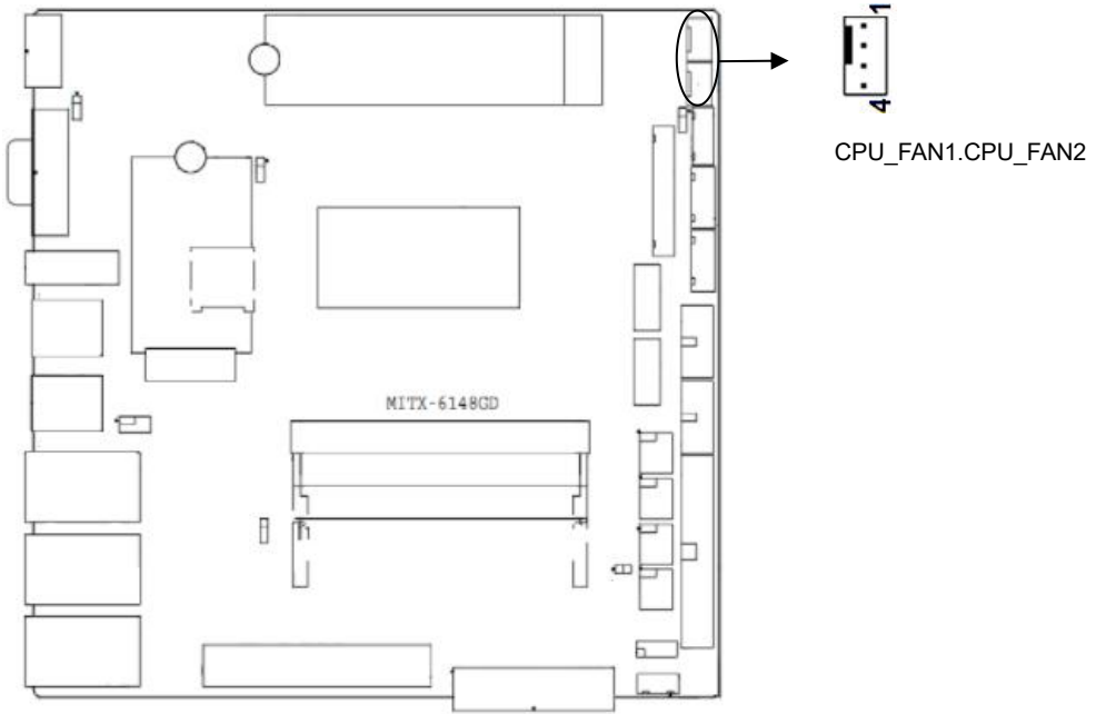
CPU_FAN1.CPU_FAN2:
